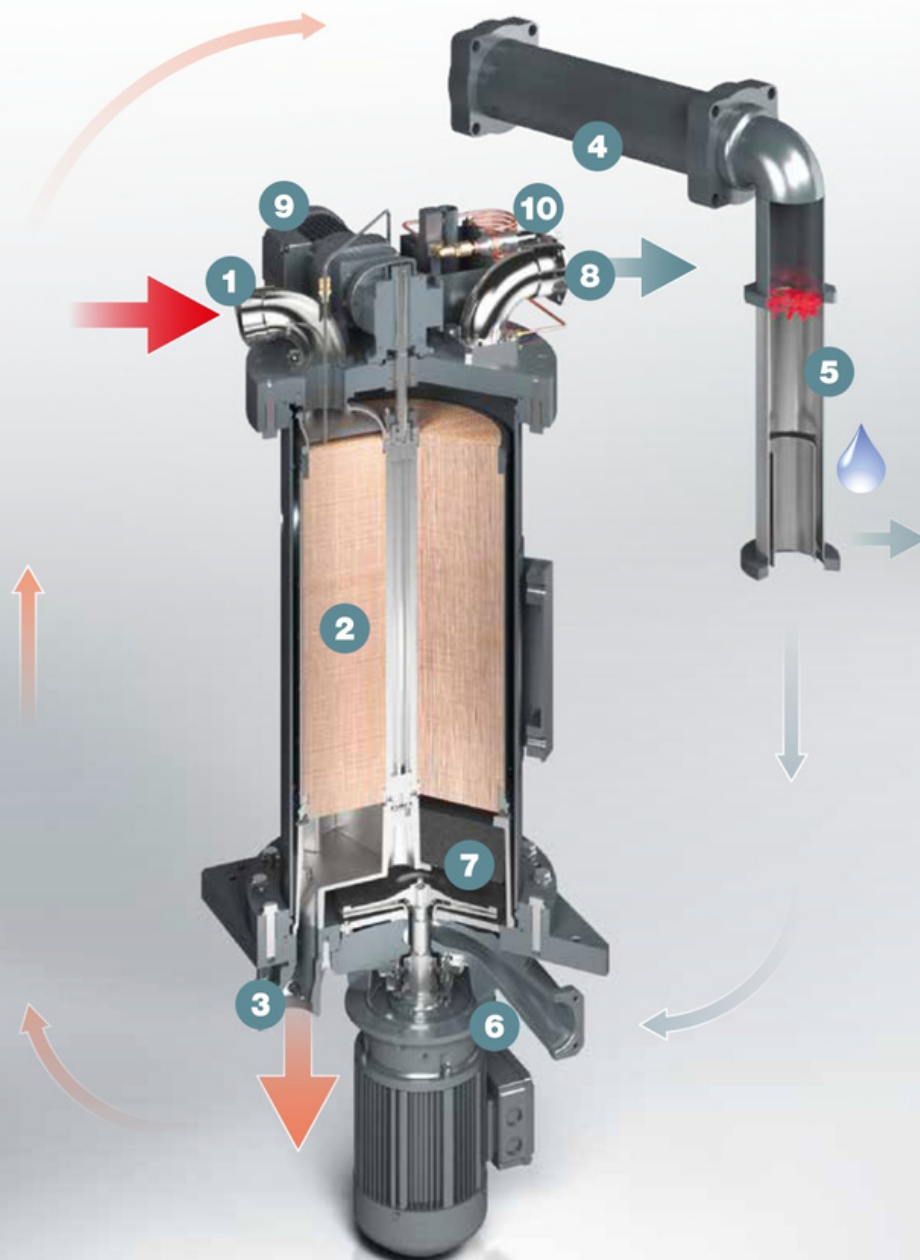
Image: RD 130 rotation dryer
