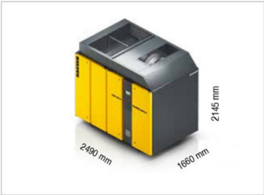
Versions with rotation dryer
